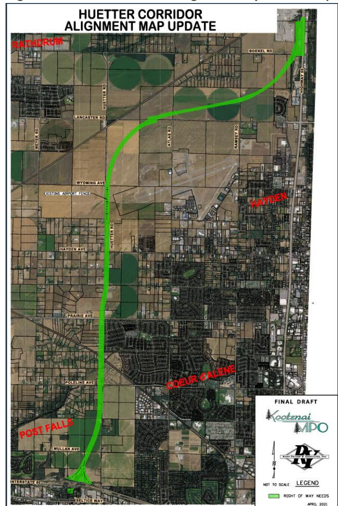
Figure 1.3 Huetter Corridor Right-of-Way Needs Map
