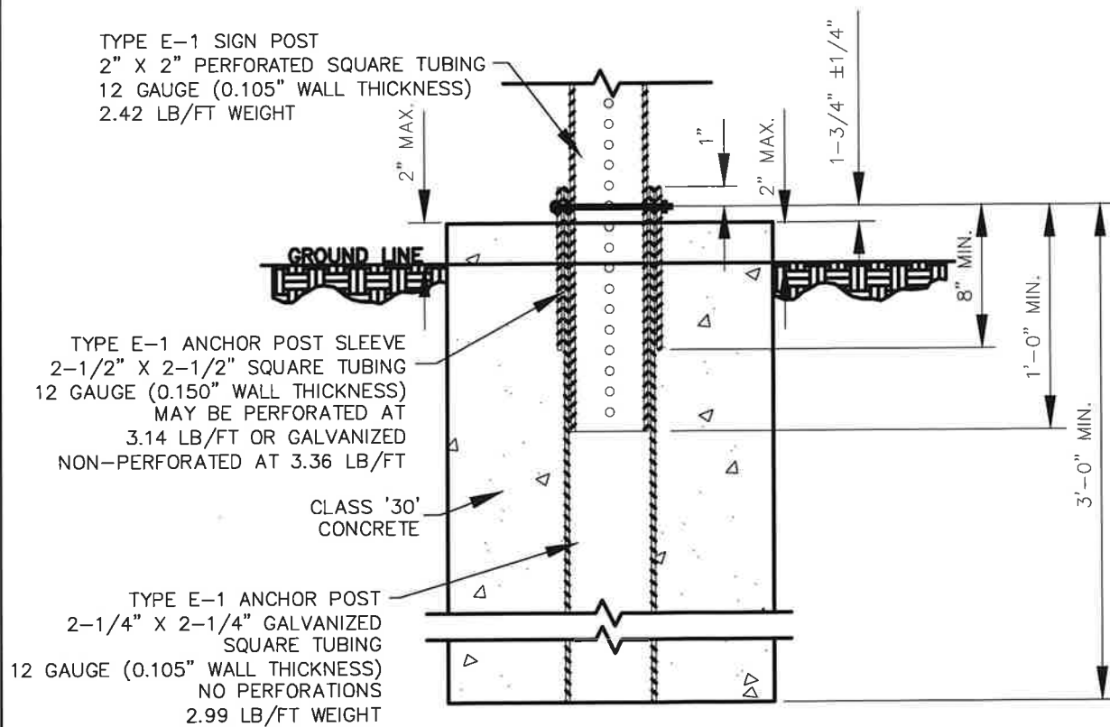
TYPE E-1 SIGN POST SECTION B-B
