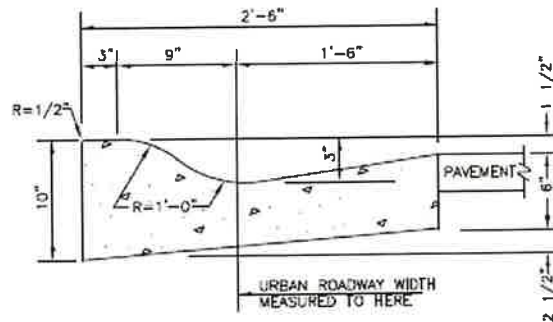
ROLL CURB ( LOCAL ROADS ONLY )
