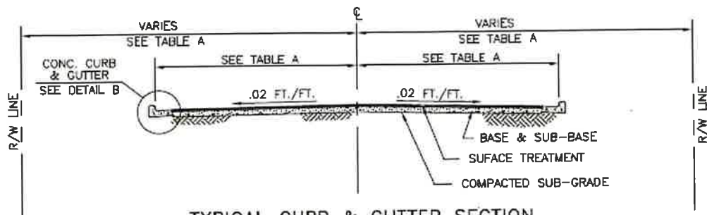
TYPICAL CURB & GUTTER SECTION N.T.S.
