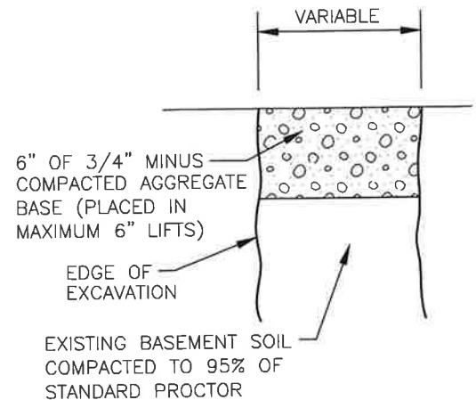
GRAVEL SURFACE
