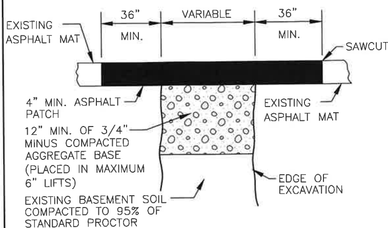
PAVED SURFACE
