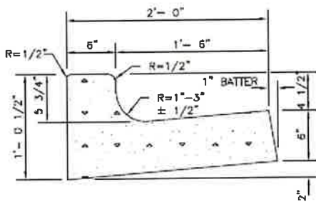
VERTICAL CURB
